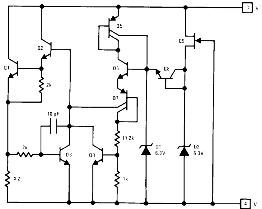
Temperature Stabilizer
